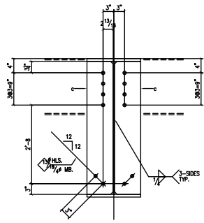
SECT. B
