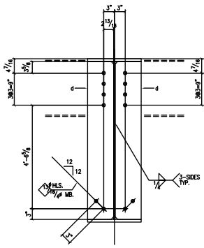
SECT. C
